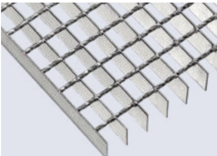
Forge welded gratings Mesh 38 x 38
